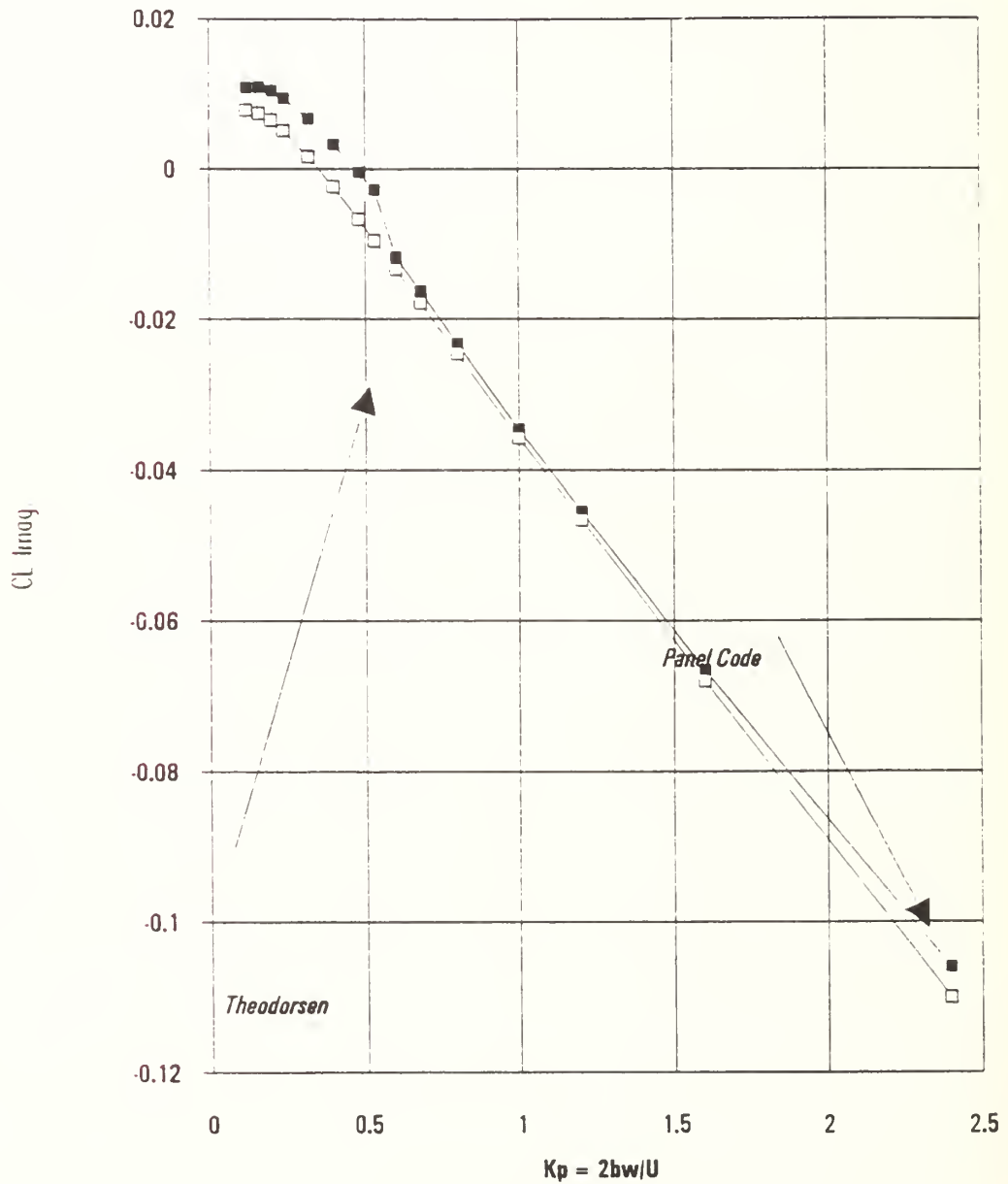
Imag. Part of C_l for Panel and Theodorsen (pitch, 1.0 deg, .37c, NACA0007, 75 panels top and bottom, 3cycles of 65 calc. per cycle)
